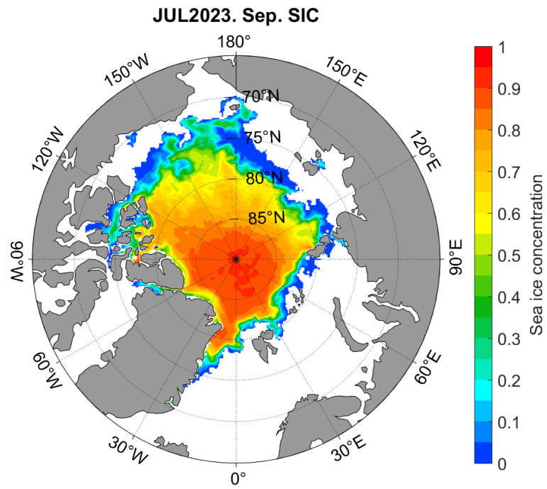
Figure s1. Spatial pattern of the predicted September-mean sea ice concentration (SIC).
