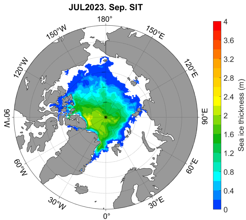
Figure s2. Spatial pattern of the predicted September-mean sea ice thickness (SIT).
